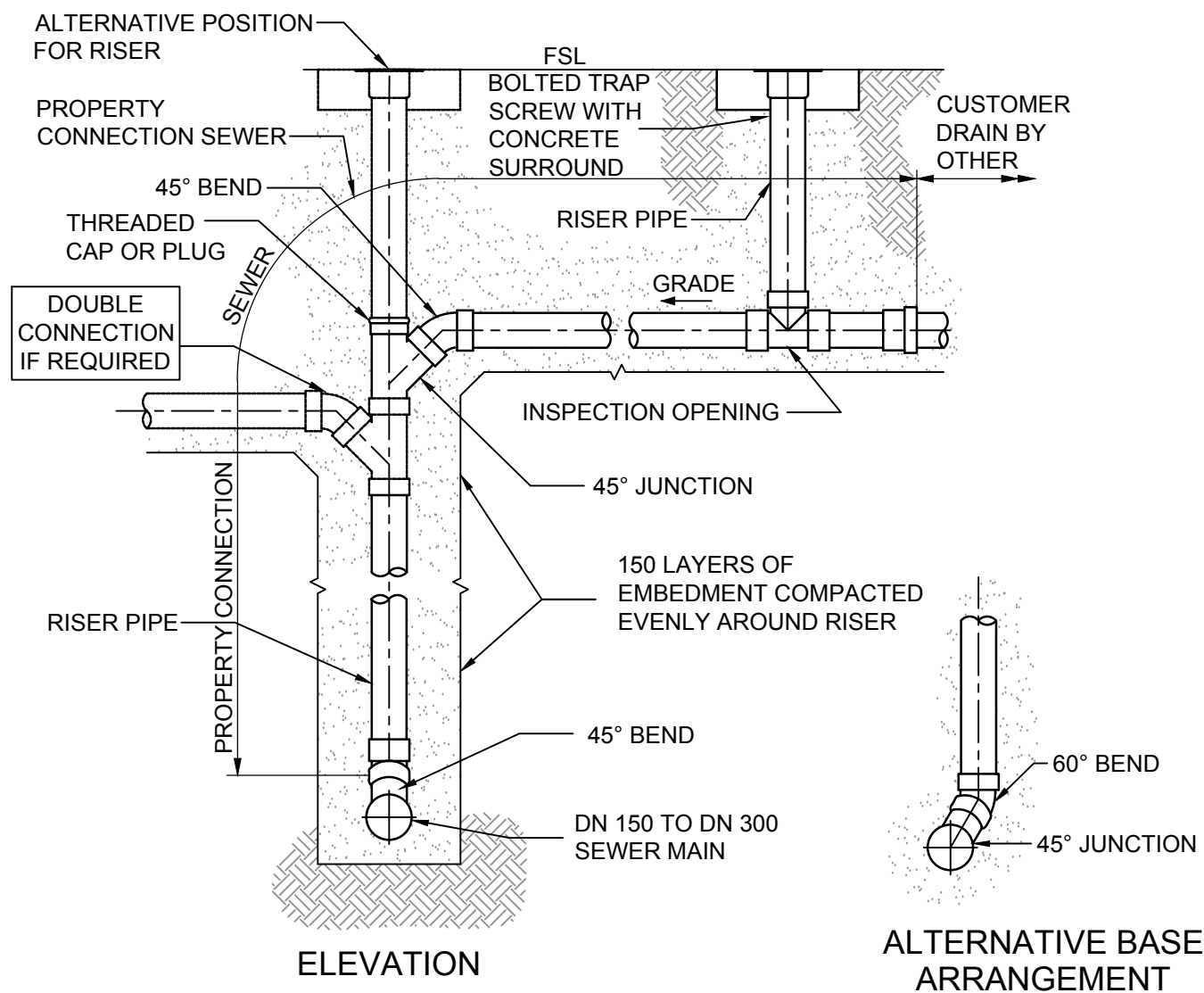
VERTICAL RISER WITH SINGLE OR DOUBLE CONNECTION (MAY BE USED WHEN VERTICAL DROP > 1200)
