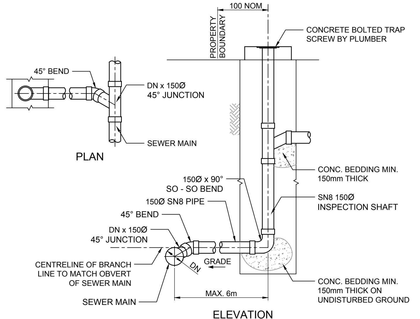
DEEP SEWER JUNCTION TO SIDE OF MAIN (>1.2m) MARK AS "V" ON W.A.E
