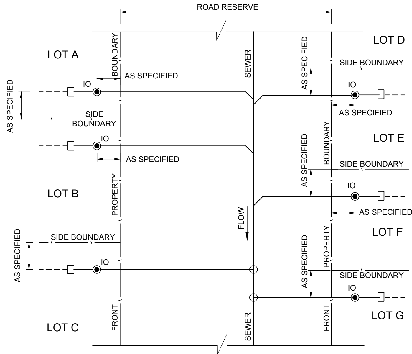
INSPECTION OPENING (IO) INTERFACE METHOD
